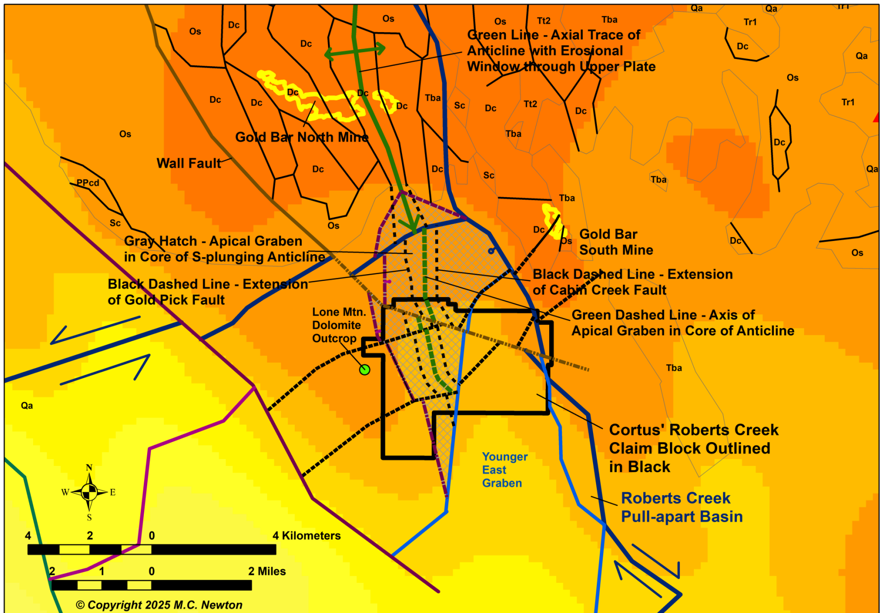
Figure 9. Regional complete Bouguer gravity anomaly. Orange - gravity highs (shallow bedrock), yellow – gravity lows (deep alluvium). Note two gravity highs in the basin, bedrock extensions from range, flank a trough of lower gravity indicating a graben in the core region of a SSE-plunging anticline.
