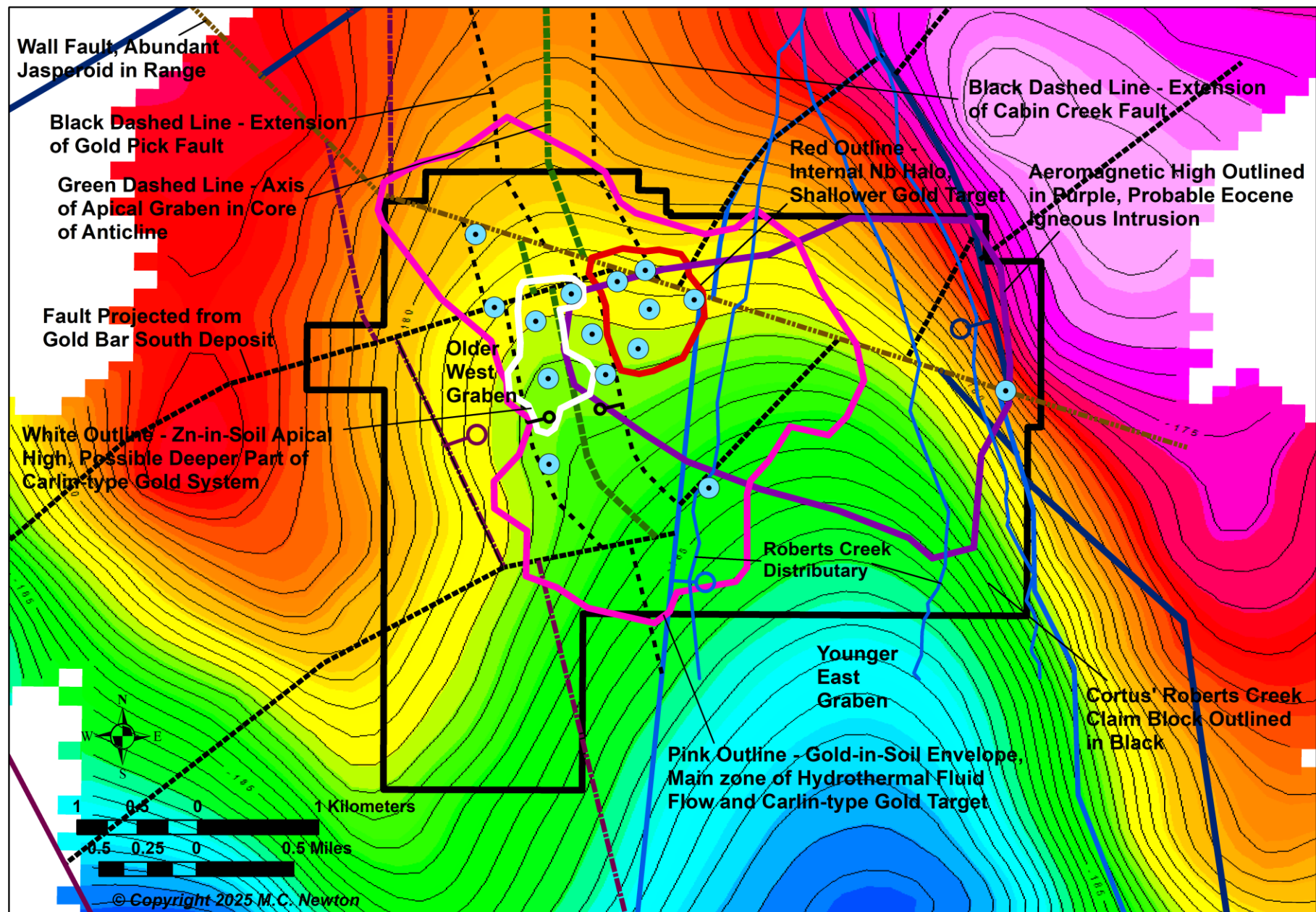
Figure 21. Detailed gravity – Red/purple highs, blue lows. Zones of high gravity anomalies are probably buried ridges of shallower bedrock. Shallower gold target on a ridge outlined in red, deeper gold target outlined in white. First 15 planned drill holes in blue circles.
