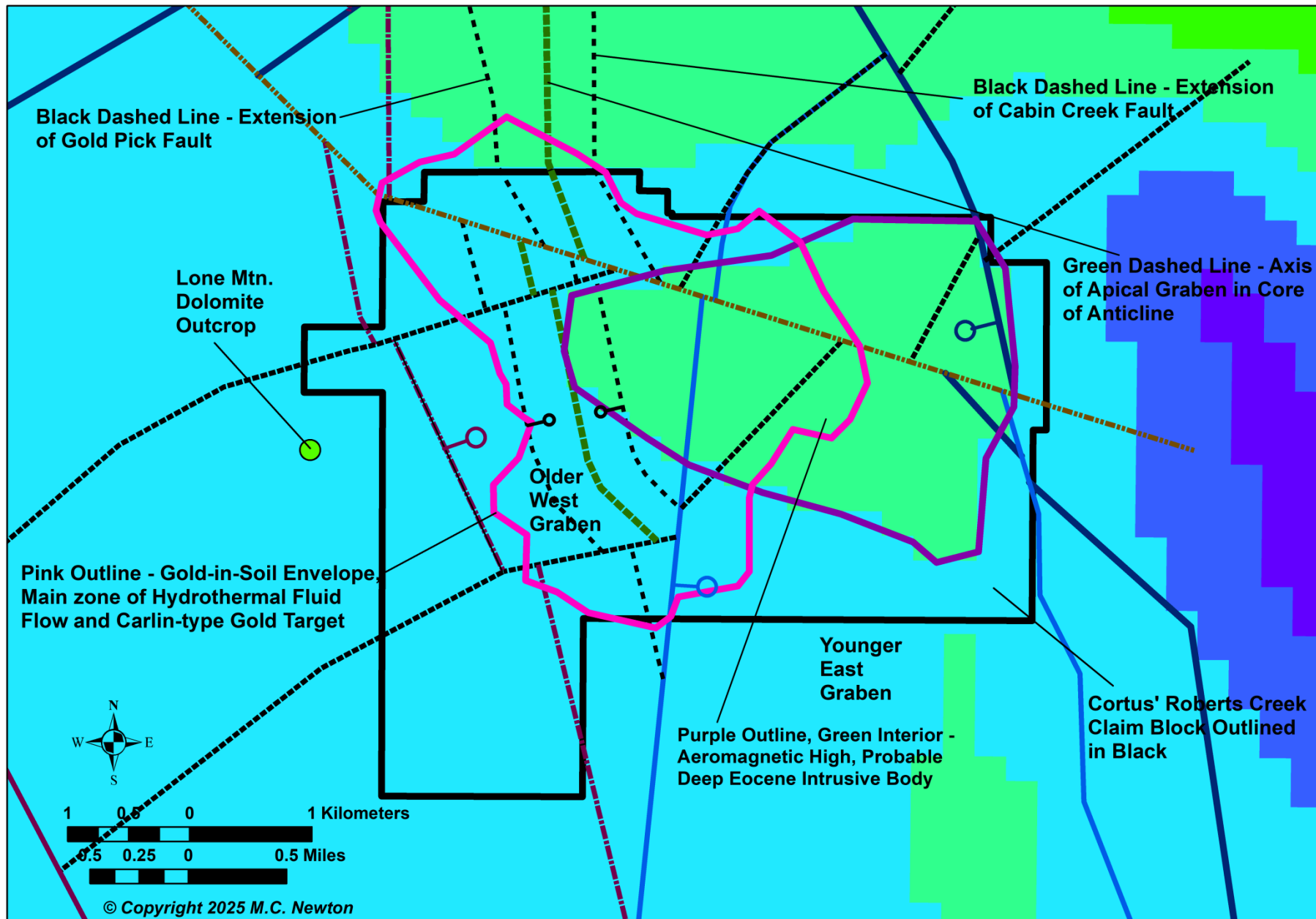
Figure 13. Aeromagnetic map. Green – magnetic highs, blue - magnetic lows. The magnetic high (in green outlined in purple) is probably a buried igneous intrusion of Eocene age. This body would have provided heat and metals to hydrothermal fluids that would have flowed upward into fractured bedrock (in pink outline).
