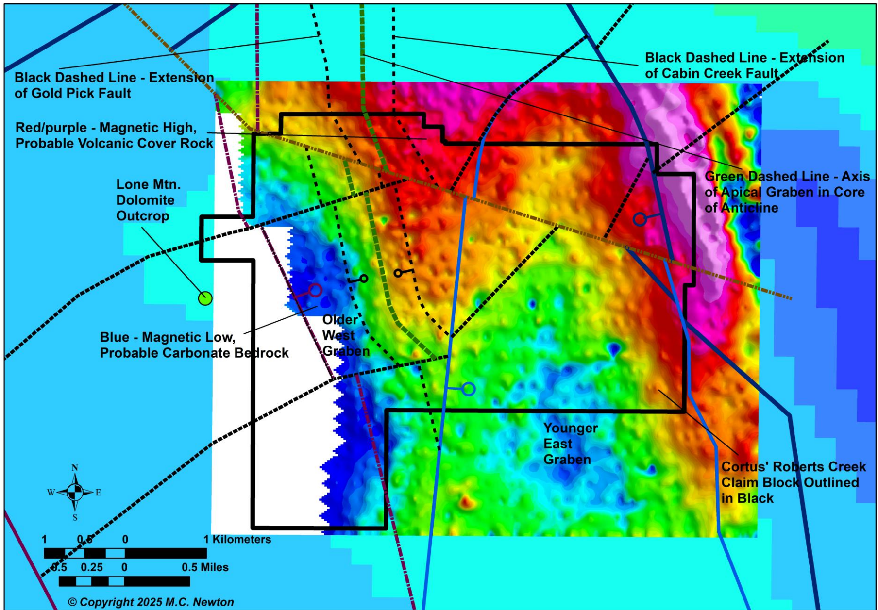
Figure 12. Overlay of ground residual magnetic intensity (reduced to pole) on regional aeromagnetic map. Red/purple - magnetic highs, blue - magnetic lows. The ground magnetics are seeing shallow bedrock and cover. Red to green regions are probably volcanic cover rocks, possibly Miocene basalt, thinning to west and dropped down in the south.
