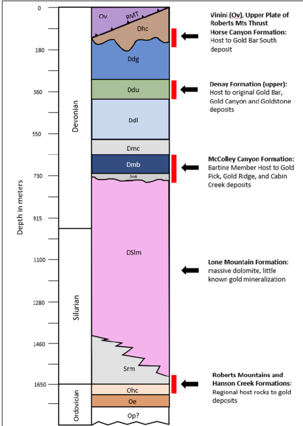
Figure 11. Stratigraphic column for Gold Bar area showing known positions of gold mineralization as red bars. After Kastelic, et al., 2020.
