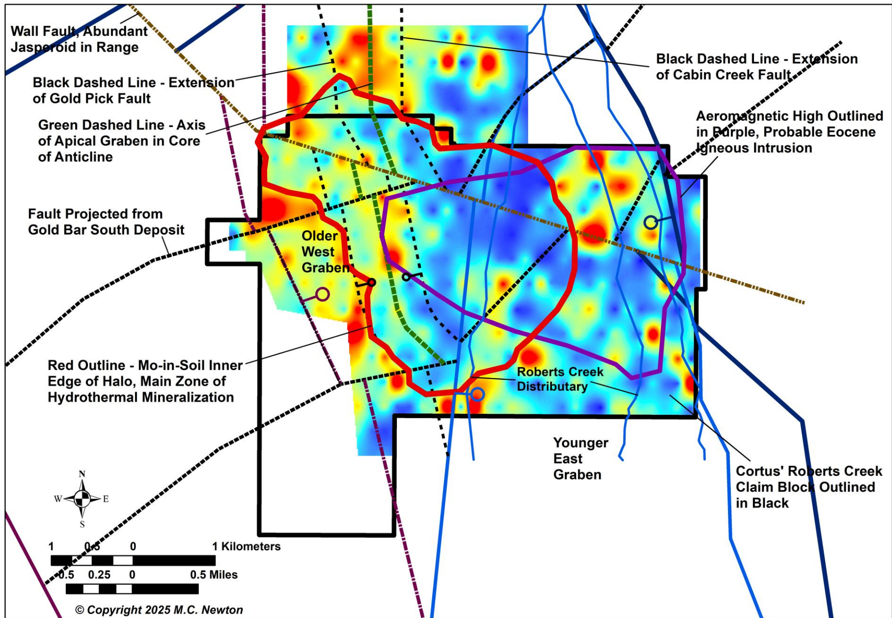
Figure 14. Molybdenum (Mo) in soil by Ionic Leach – red highs, blue lows. Note halo of scattered strong Mo highs outside red outline. This may be defining the outside of the main hydrothermal alteration system.
