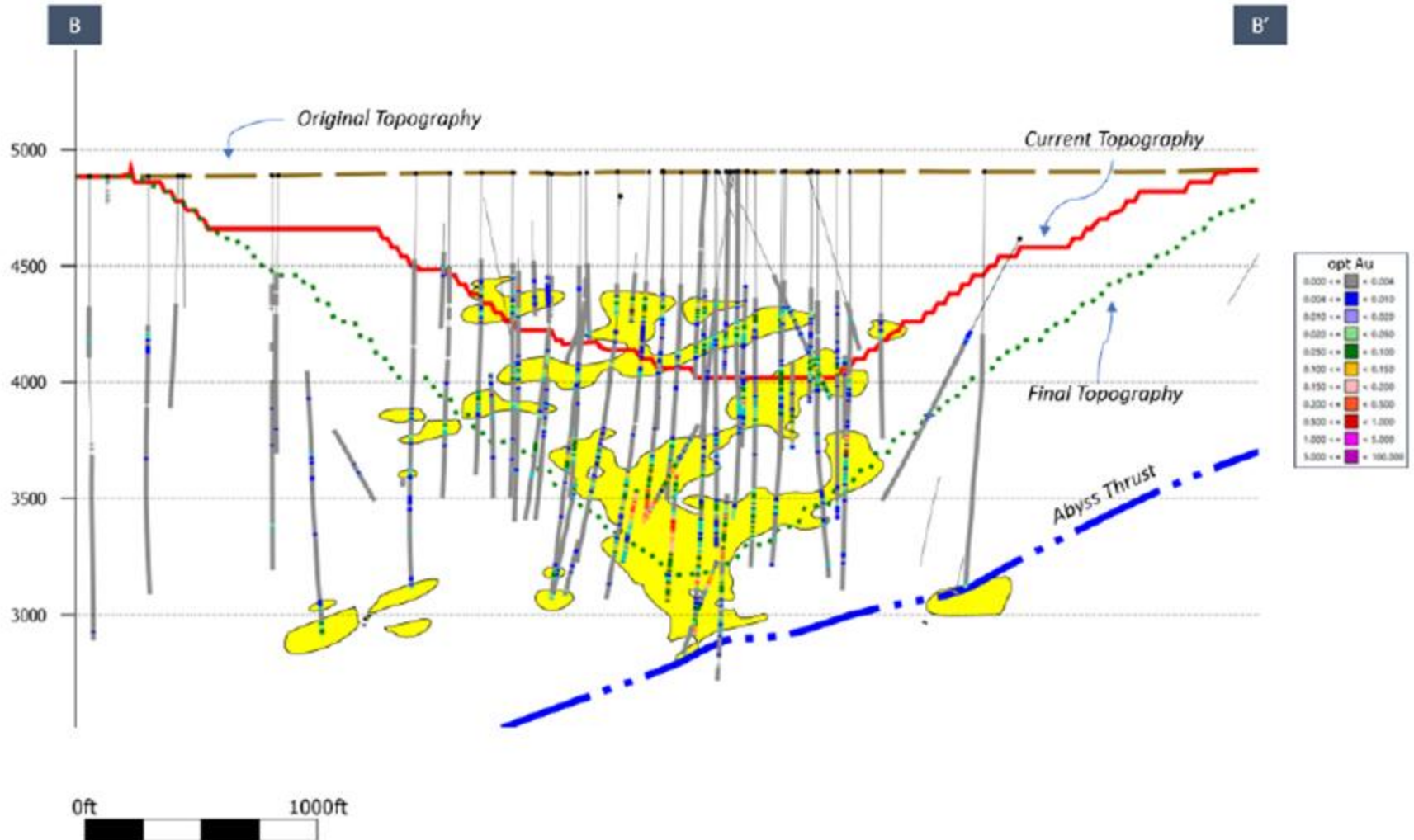
Figure 7-12: Cross-Section, Crossroads
