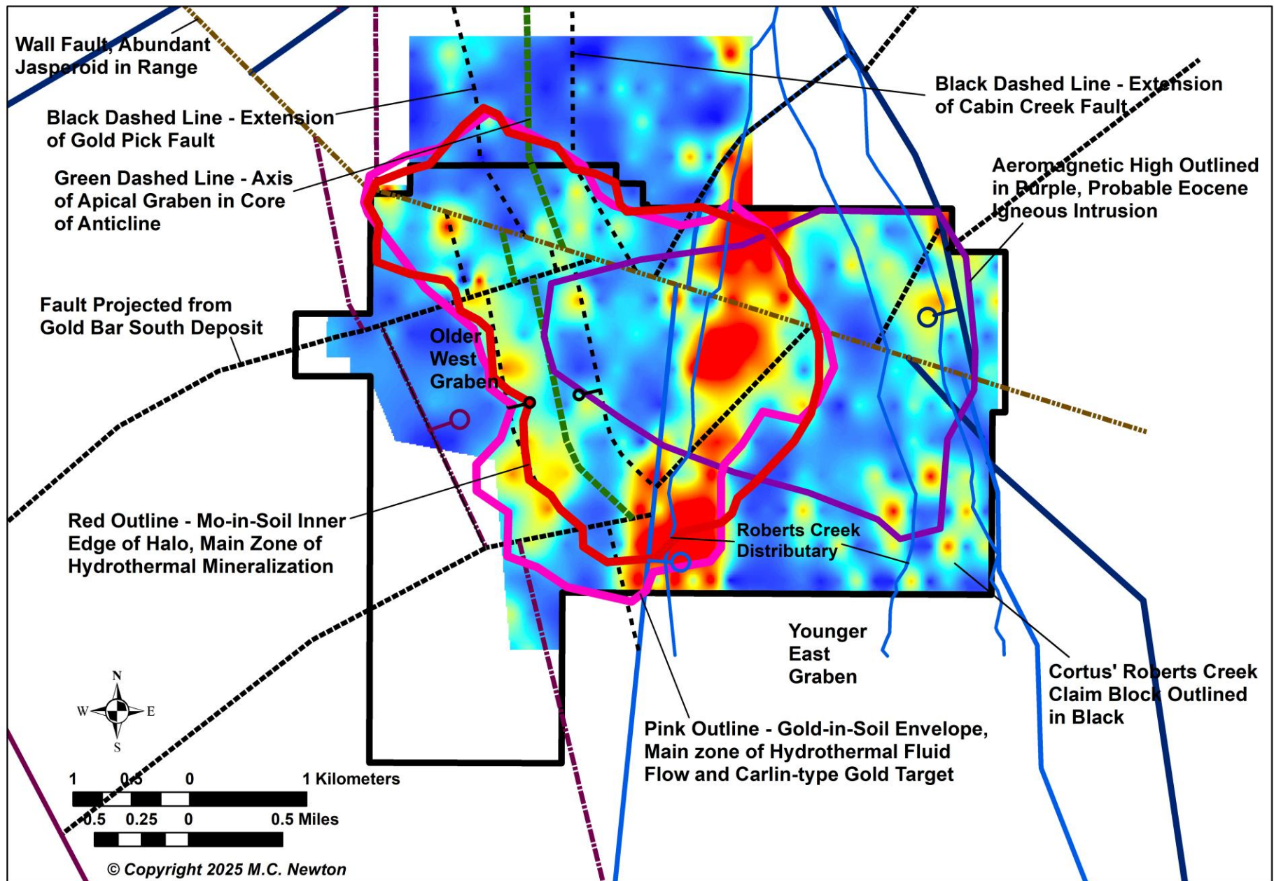
Figure 15. Gold (Au) in soil by Ionic Leach – red highs, blue lows. Pink line is envelope around gold highs – roughly coincident with Mo halo (red line). Western Au high anomaly along projected faults from Gold Bar North and South deposits. Central strong linear anomaly probably mainly due to stream sediment with contribution of gold from below.
