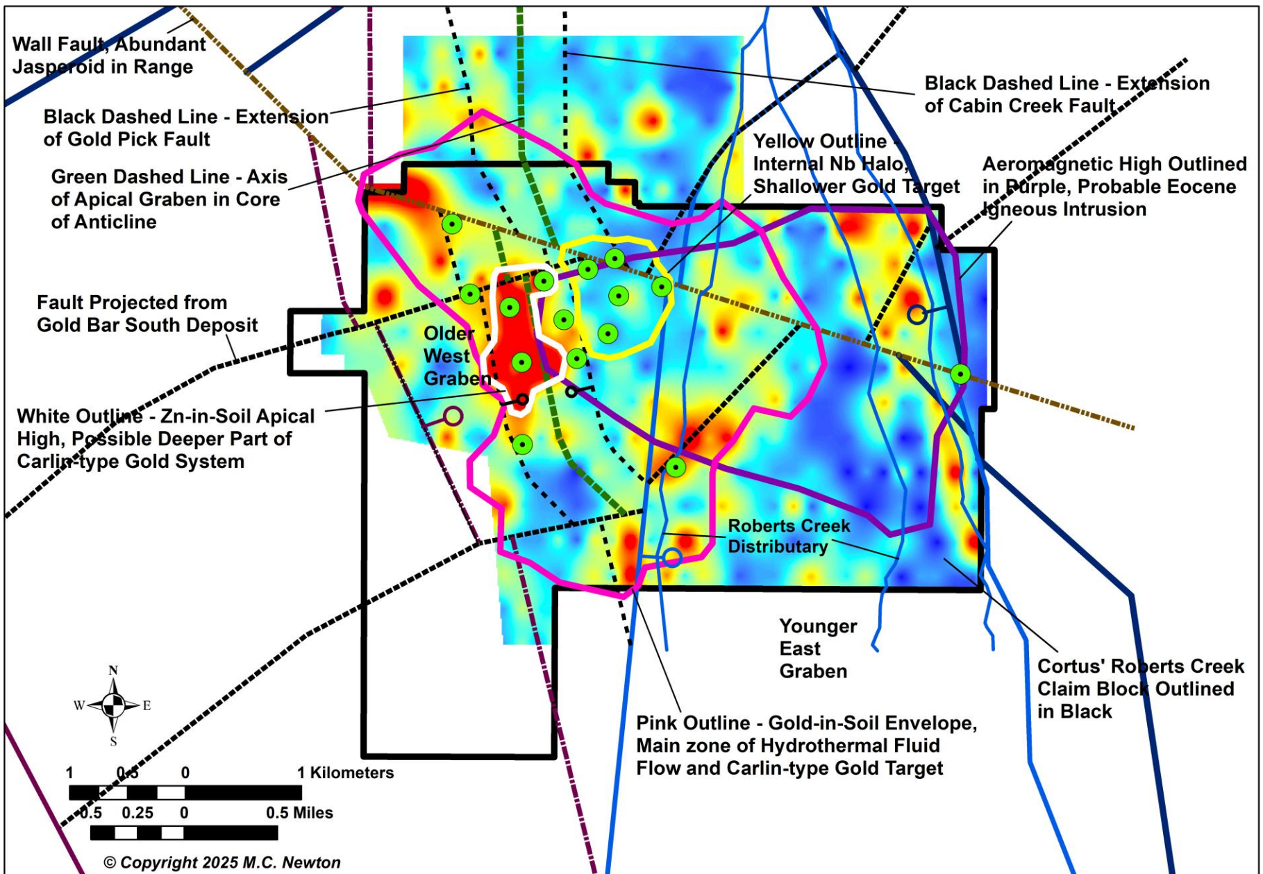
Figure 18. Zinc (Zn) in soil by Ionic Leach – red highs, blue lows. Strong Zn high anomaly (outlined in white) is probably apical – directly above mineralization that is deeper than target outlined in yellow. First 15 planned drill holes in green circles.
