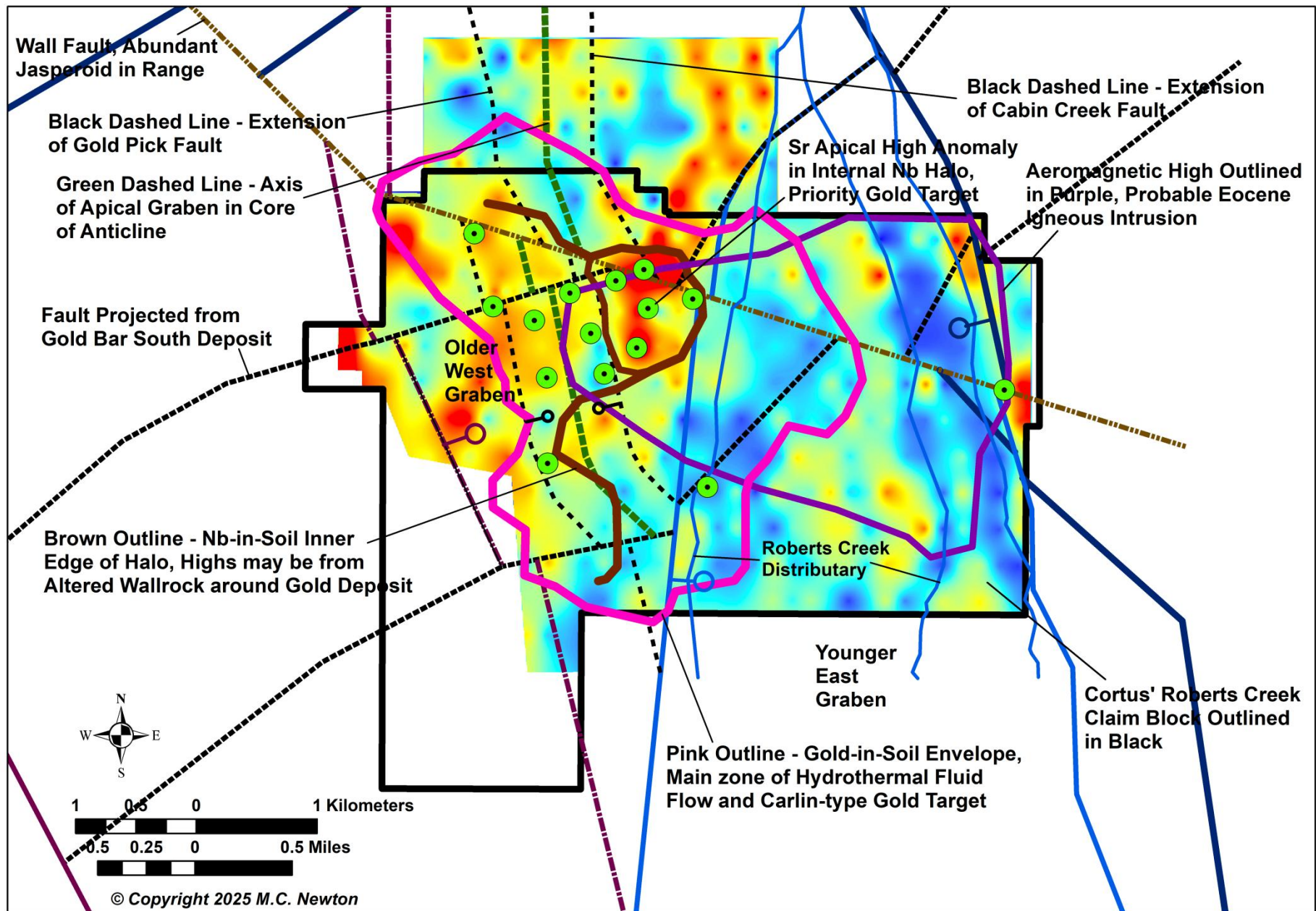
Figure 17. Strontium (Sr) in soil by Ionic Leach – red highs, blue lows. Note strong Sr high anomaly inside inner Nb halo (brown) – possible Sr apical anomaly suggesting carbonate dissolution. First 15 planned drill holes in green circles.
